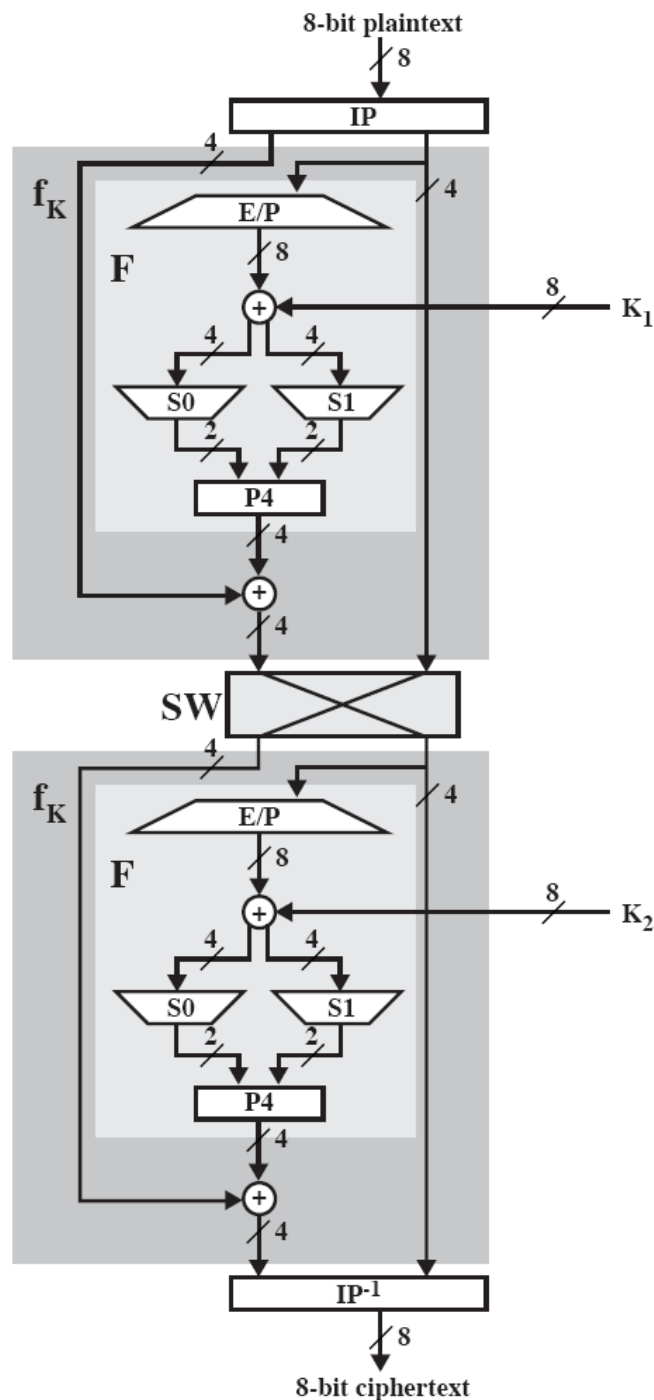
Figure 3.3 Simplified DES Encryption Detail
