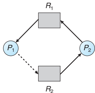
Figure 7.8 An unsafe state in a resource-allocation graph.
