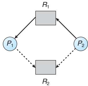
Figure 7.7 Resource-allocation graph for deadlock avoidance.
